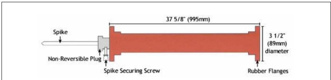
Figure A.3 —Dimensions of fixed depth searcher bar
