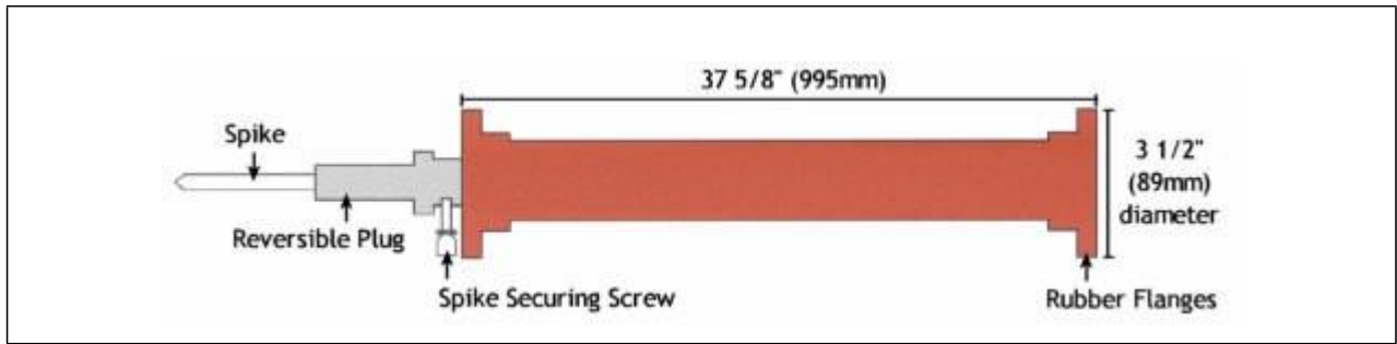
Figure A.2 —Dimensions of adjustable depth searcher bar
